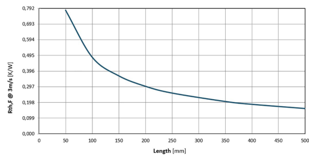
Thermal Resistance - Forced convection
