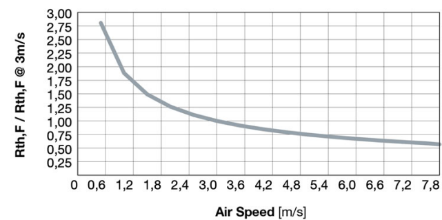
Air speed correction factor
