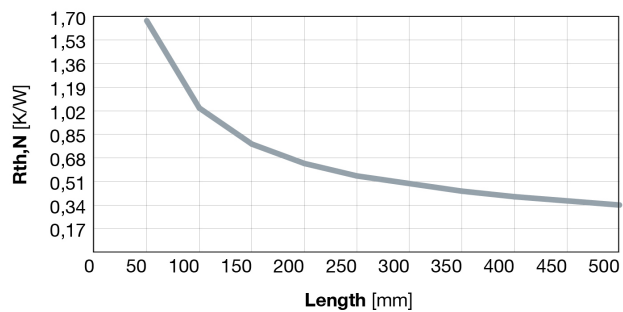
Thermal Resistance - Natural convection
