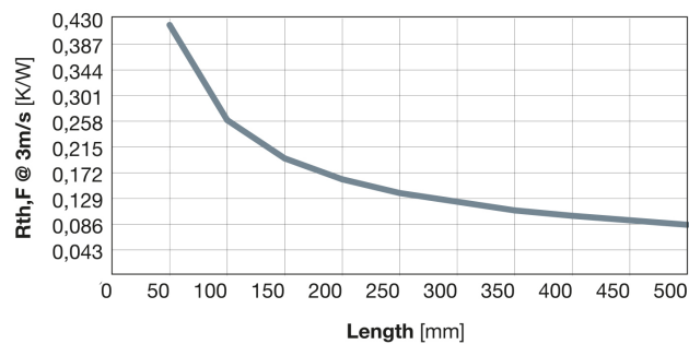
Thermal Resistance - Forced convection
