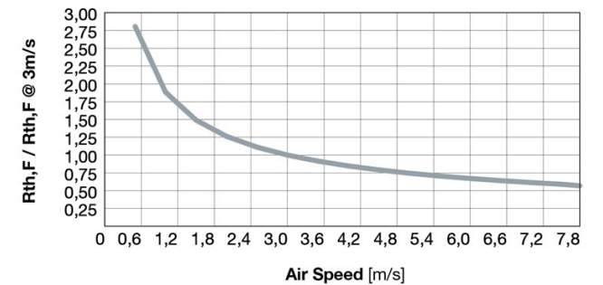
Air speed correction factor
